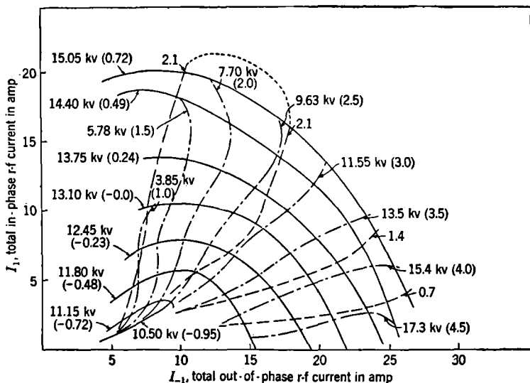
FIG. 6-11.—Average energy loss per electron (in reduced units) at constant magnetic field with ——— d-c voltage contours in kv, - - - r-f voltage contours in kv, ····· electron loss in kv. Figures in parentheses are reduced voltages; d-c values relative to threshold. Reduced linear current densities are given by I/36 .
